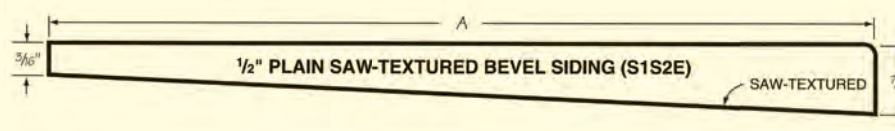
1/2x8 PATTERN #323R PLAIN BEVEL
