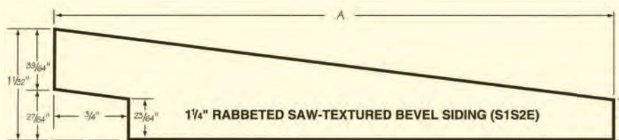
1 1/4x8 PATTERN #477 THICK BUTT BEVEL
