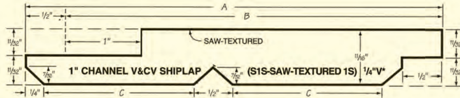
1x6 PATTERN #784R CHANNEL V & CV SHIPLAP
