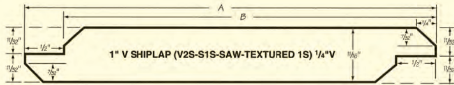
1x8 PATTERN #794R SHIPLAP
