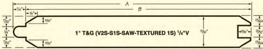
1x6 PATTERN #711R T&G 1x8 PATTERN #712R T&G
